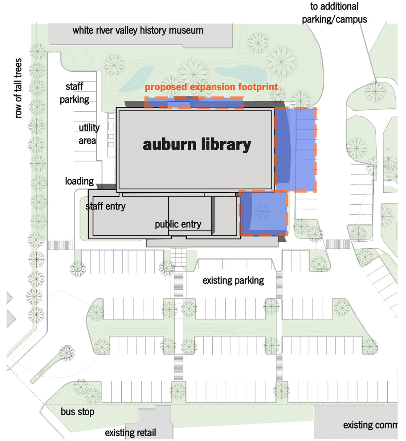
site diagram - scheme B (3.1) 1"=20'
